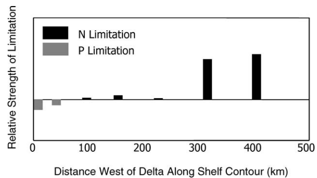
Fig. 3. Simulated changes in the nitrogen and phosphorus limitations along shelf contour between the Mississippi River Delta and the Texas Coast during July 1990 (from Limno-Tech, Inc. 1995).
