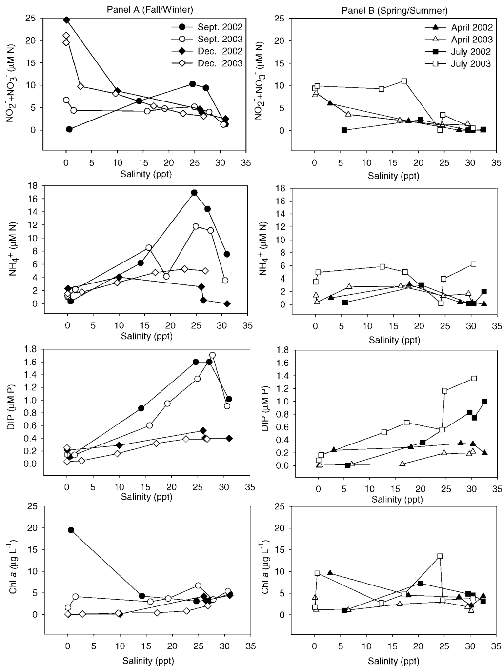
Figure 5. Representative seasonal distributions of dissolved nitrite plus nitrate ( \text{NO}_2 + \text{NO}_3 ), ammonium ( \text{NH}_4^+ ), inorganic phosphorus (DIP), and chlorophyll a (Chl a ) vs. salinity in the Mullica River–Great Bay Estuary, New Jersey, from 2002 to 2003. Note that Panel A in the left column contains distributions from fall and winter, and Panel B in the right column contains distributions from spring and summer.
